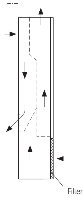
Routing of air flow
