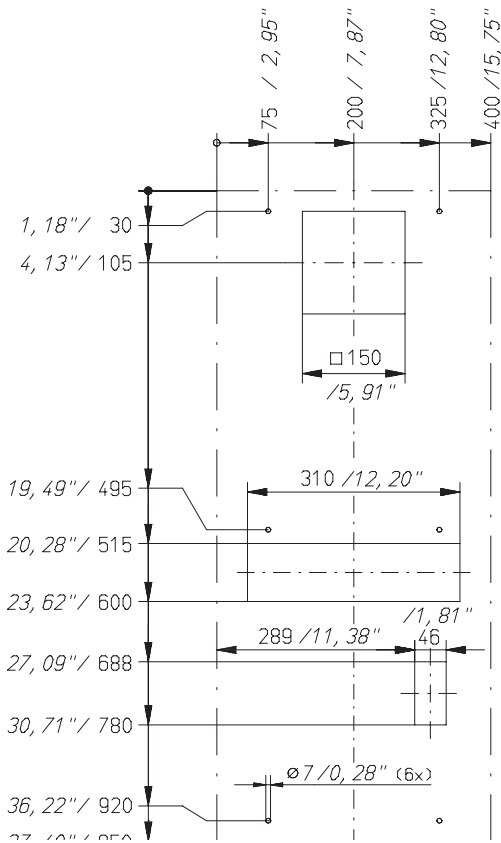
Drilling template external mounting
